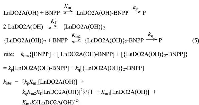
Scheme 4. A monomer-dimer saturation reaction model.
