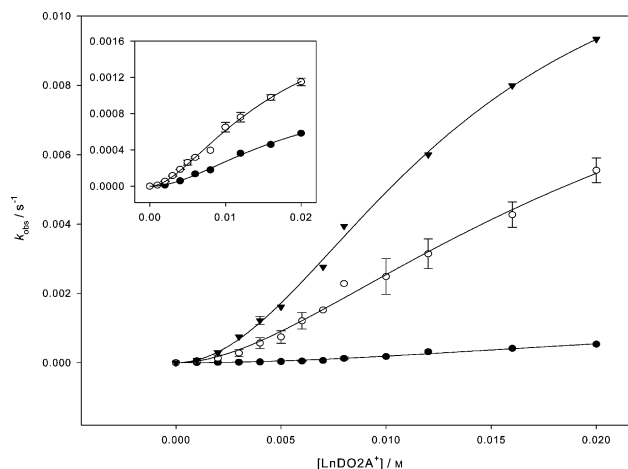
Figure 4. Plots of the pseudo-first-order rate constants of BNPP hydrolysis vs. the concentration of \text{LnDO2A}^+ . EuDO2A + : (●) pH 7.90, (○) pH 9.35, (▼) pH 9.90. Inset: ErDO2A + : (●) pH 9.90 and YbDO2A + : (○) pH 9.90. 25 °C, [\text{BNPP}] = 0.10 \text{ mM} , [\text{buffer}] = 20 \text{ mM} , \mu = 0.10 \text{ M} (\text{CH}_3)_4\text{NCl} . The solid lines were calculated based on the best non-linear least-squares fits according to the monomer-dimer saturation reaction model in Scheme 4.
