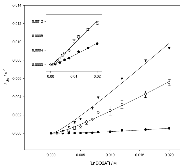
Figure 3. Plots of the pseudo-first-order rate constants of BNPP hydrolysis vs. the concentration of \text{LnDO}_2\text{A}^+ : \text{EuDO}_2\text{A}^+ : (●) pH 7.90, (○) pH 9.35, (▼) pH 9.90. Inset: \text{ErDO}_2\text{A}^+ : (●) pH 9.90 and \text{YbDO}_2\text{A}^+ (○) pH 9.90. 25 °C, [\text{BNPP}] = 0.10 \text{ mM} , [\text{buffer}] = 20 \text{ mM} , \mu = 0.10 \text{ M} (\text{CH}_3)_4\text{NCl} . The solid lines were calculated based on the best non-linear least-squares fits according to the monomer-dimer reaction model shown in Scheme 2.
