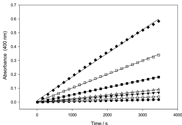
Figure 1. Plots of absorbance at 400 nm vs. time (s) for the \text{EuDO}_2\text{A}^+ -promoted BNPP hydrolysis reaction. [\text{EuDO}_2\text{A}^+] = 1.0 \text{ mM} ; [\text{BNPP}] = 0.2 (●), 0.4 (○), 0.8 (▼), 1.0 (△), 2.0 (■), 4.0 (□), 8.0 \text{ mM} (◆); 25^\circ\text{C} ; pH 7.90; [\text{MPS buffer}] = 20 \text{ mM} ; \mu = 0.10 \text{ M} (\text{CH}_3)_4\text{NCl} . Solid lines are the best fits of linear least-squares regression analyses. All r^2 values are around 1.00.
